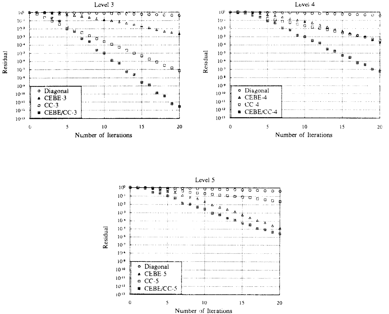
Fig. 4. Convergence histories for a two-dimensional uniform mesh with 64 \times 64 elements; Case 2.
