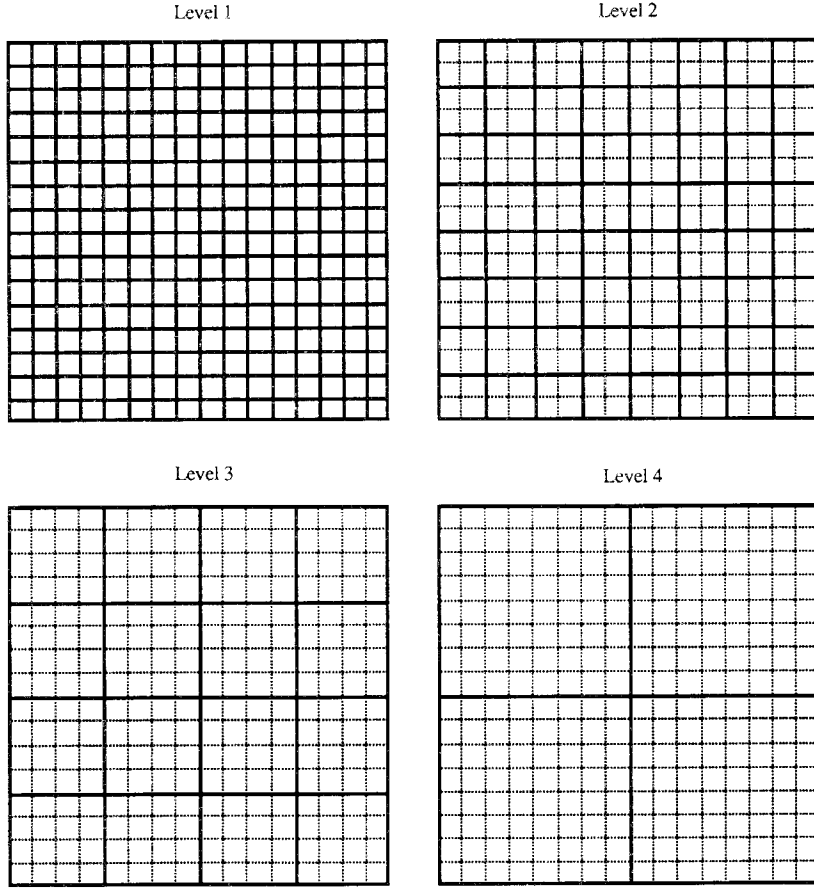
Fig. 1. Four different levels of clustering for a uniform 16 \times 16 mesh; in each frame the thick lines depict the cluster boundaries and the associated companion mesh.
