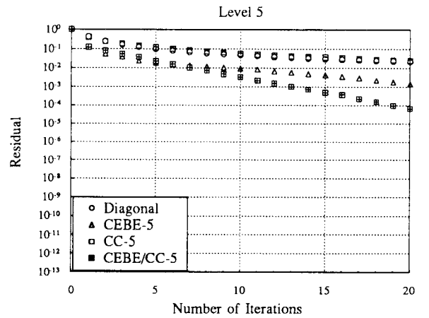
Fig. 7. Convergence histories for a two-dimensional non-uniform mesh with 256 \times 64 elements.
