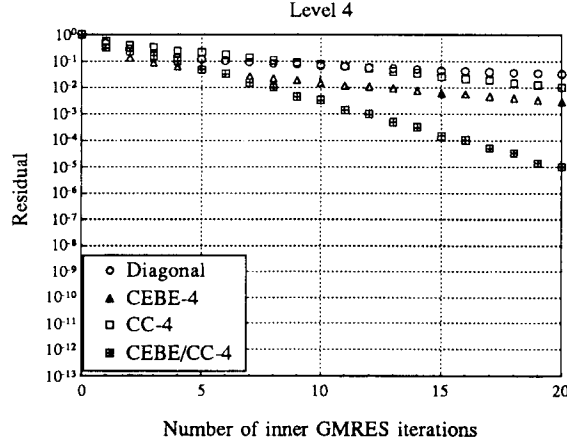
Fig. 8. Convergence histories for a three-dimensional uniform mesh with 128 \times 128 \times 64 elements.
