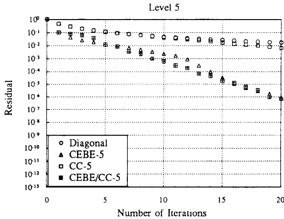
Fig. 2. Convergence histories for a two-dimensional uniform mesh with 64 \times 64 elements: Case 1.
