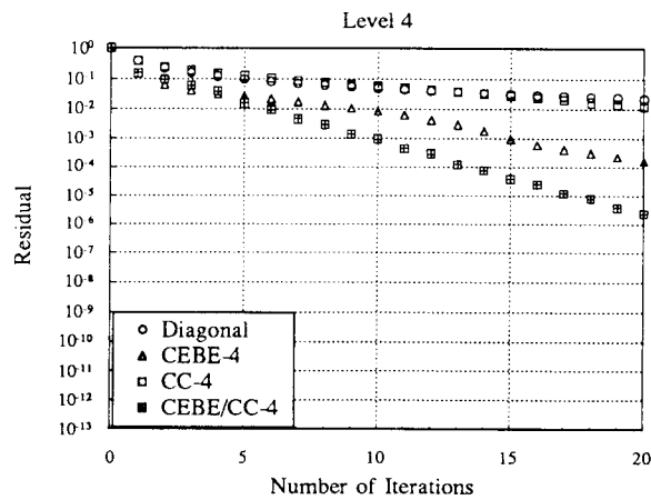
Fig. 6. Convergence histories for a two-dimensional non-uniform mesh with 128 \times 32 elements.
