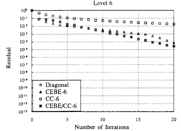
Fig. 3. Convergence histories for a two-dimensional uniform mesh with 128 \times 128 elements: Case 1.
