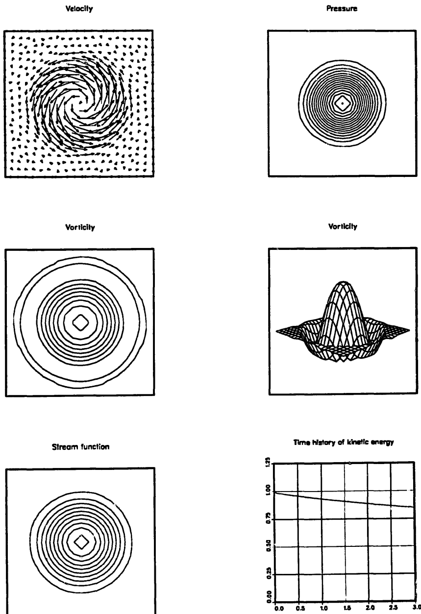
Fig. 3. Solution of the standing vortex problem at t = 3 with Q1Q1/T6.
