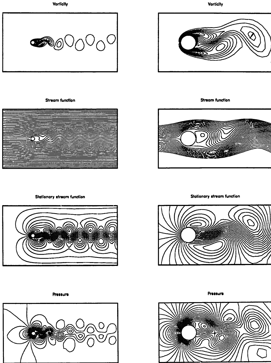
Fig. 15. Periodic solution (corresponding to the crest value of the lift coefficient) obtained with P1P1/T6.
