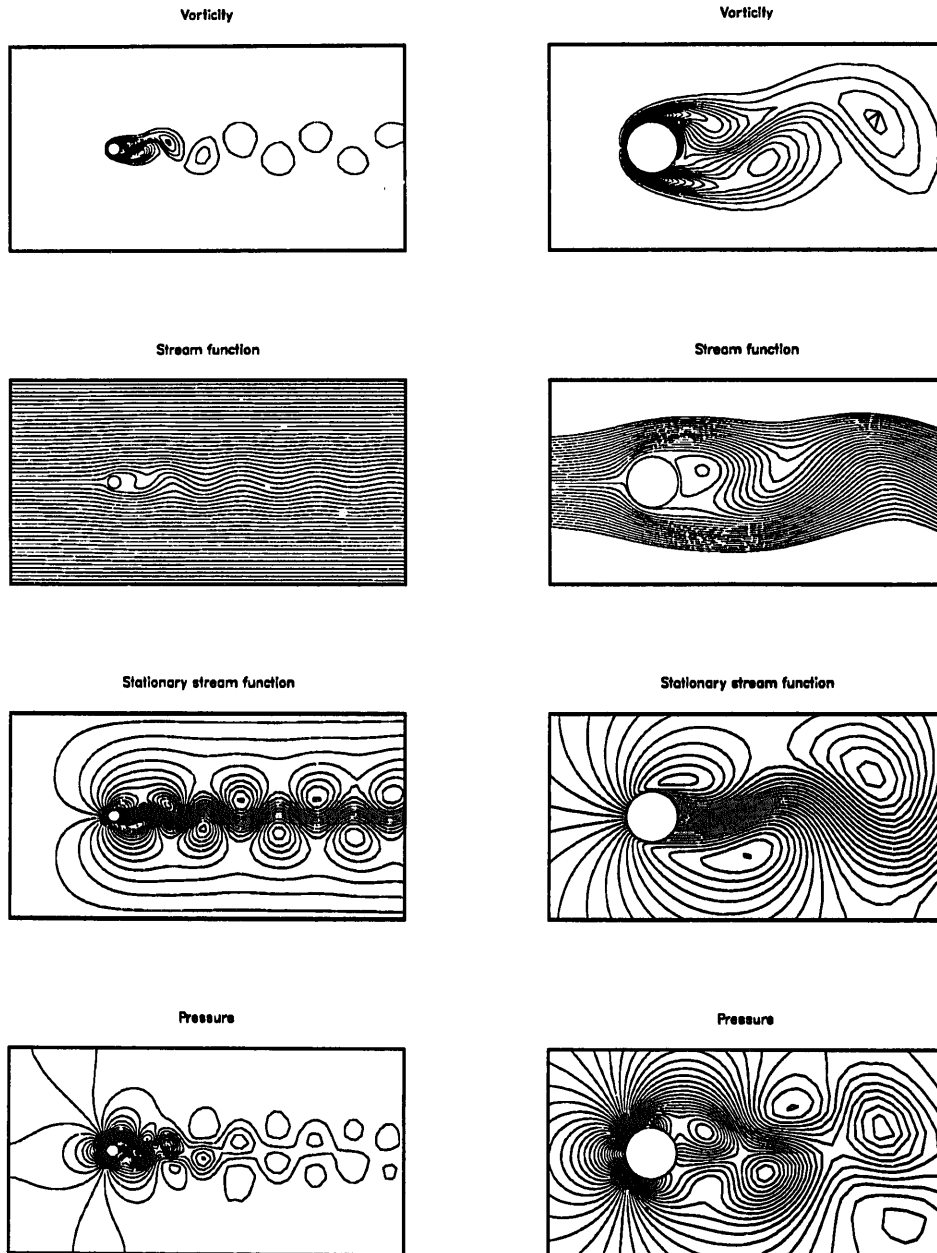
Fig. 14. Periodic solution (corresponding to the crest value of the lift coefficient) obtained with P1P1/T1
