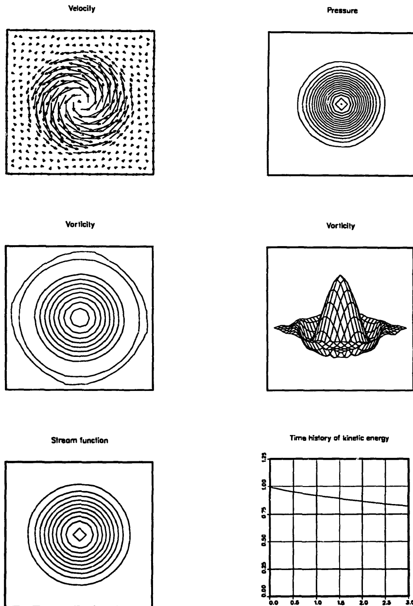
Fig. 5. Solution of the standing vortex problem at t = 3 with P1P1/T6.
