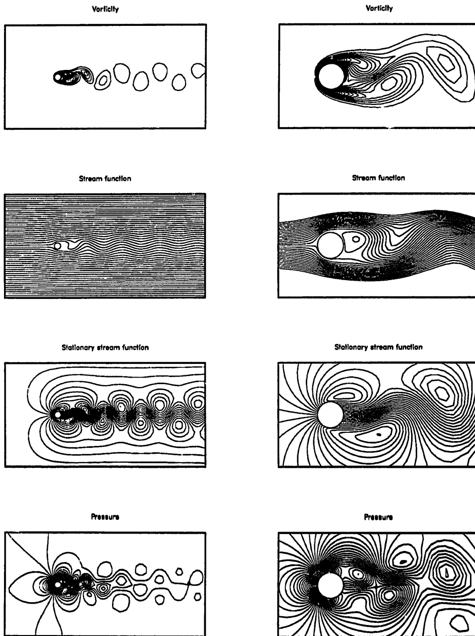
Fig. 12. Periodic solution (corresponding to the crest value of the lift coefficient) obtained with Q1Q1/T1.
