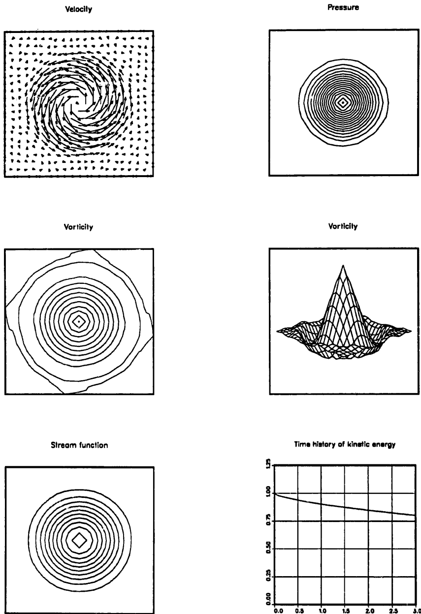
Fig. 1. Solution of the standing vortex problem at t = 3 with P1P1/T1.
