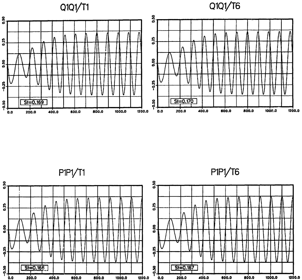
Fig. 10. Strouhal number and the time history of the lift coefficient obtained with various elements.
