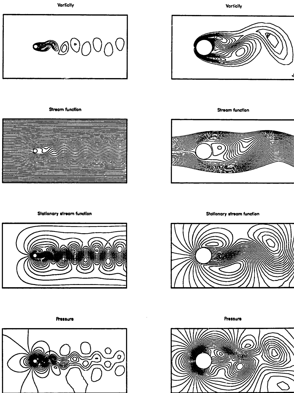
Fig. 13. Periodic solution (corresponding to the crest value of the lift coefficient) obtained with Q1Q1/T6.
