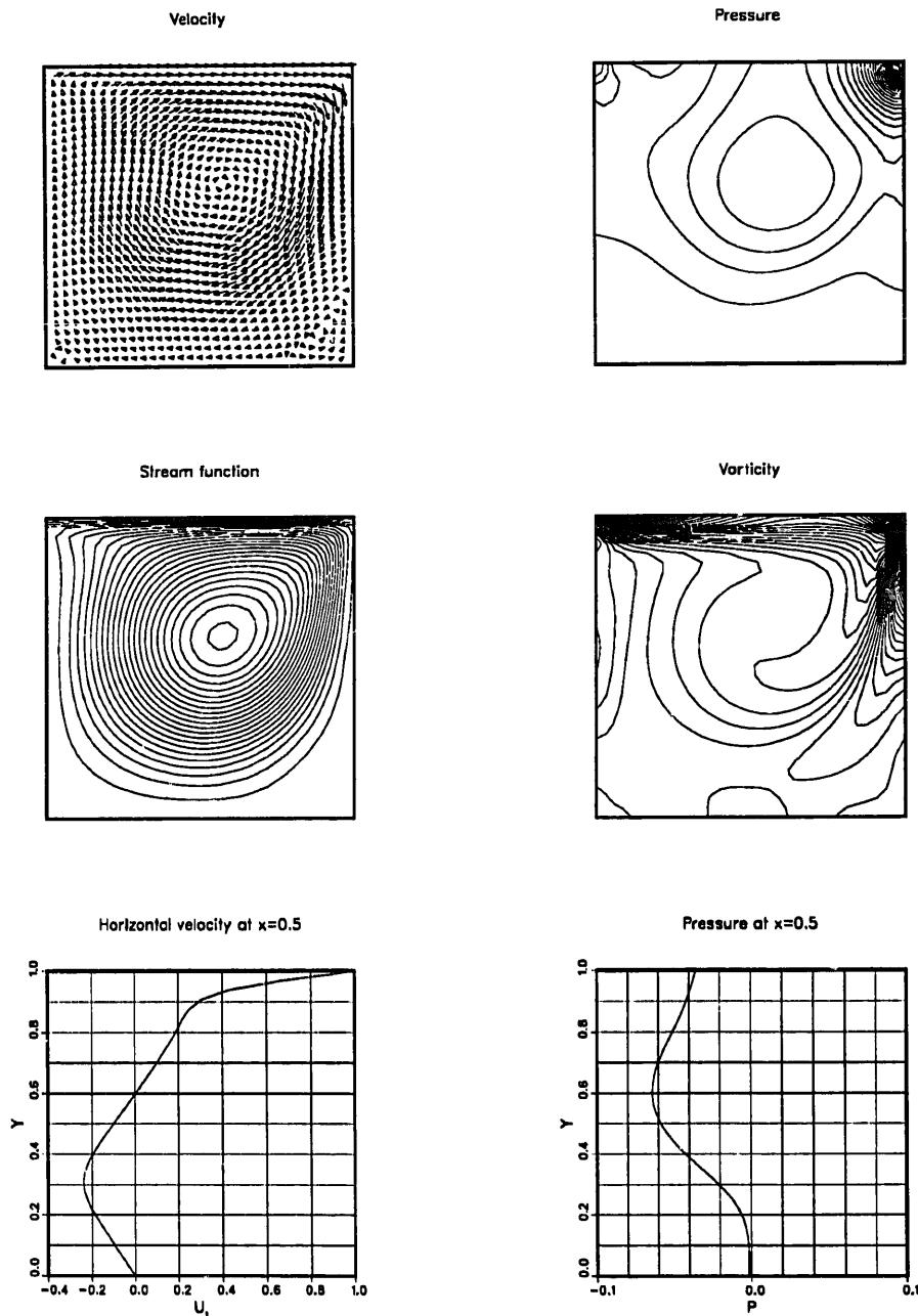
Fig. 8. Driven cavity flow at Reynolds number 400: steady-state solution obtained with Q1Q1/T1.
