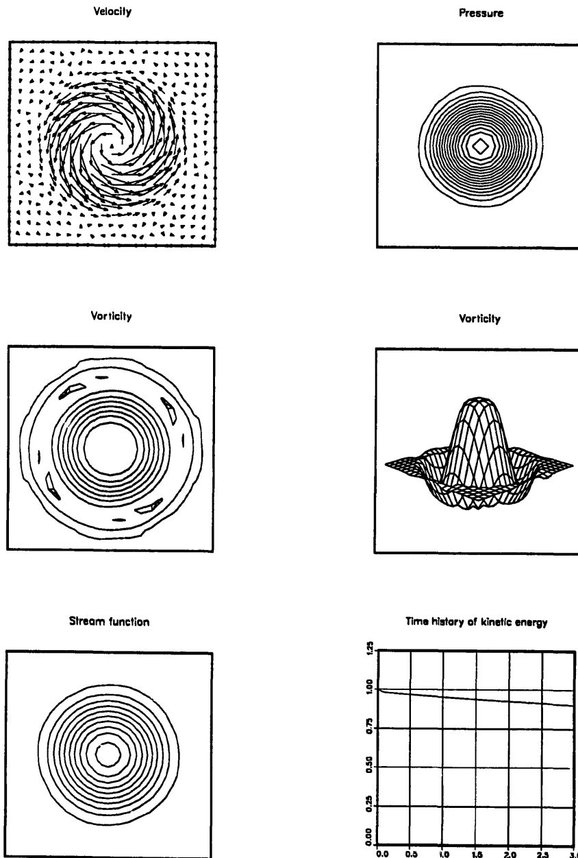
Fig. 6. Solution of the standing vortex problem at t = 3 with Q1Q1/T1 (with \tau as defined by (20)).
