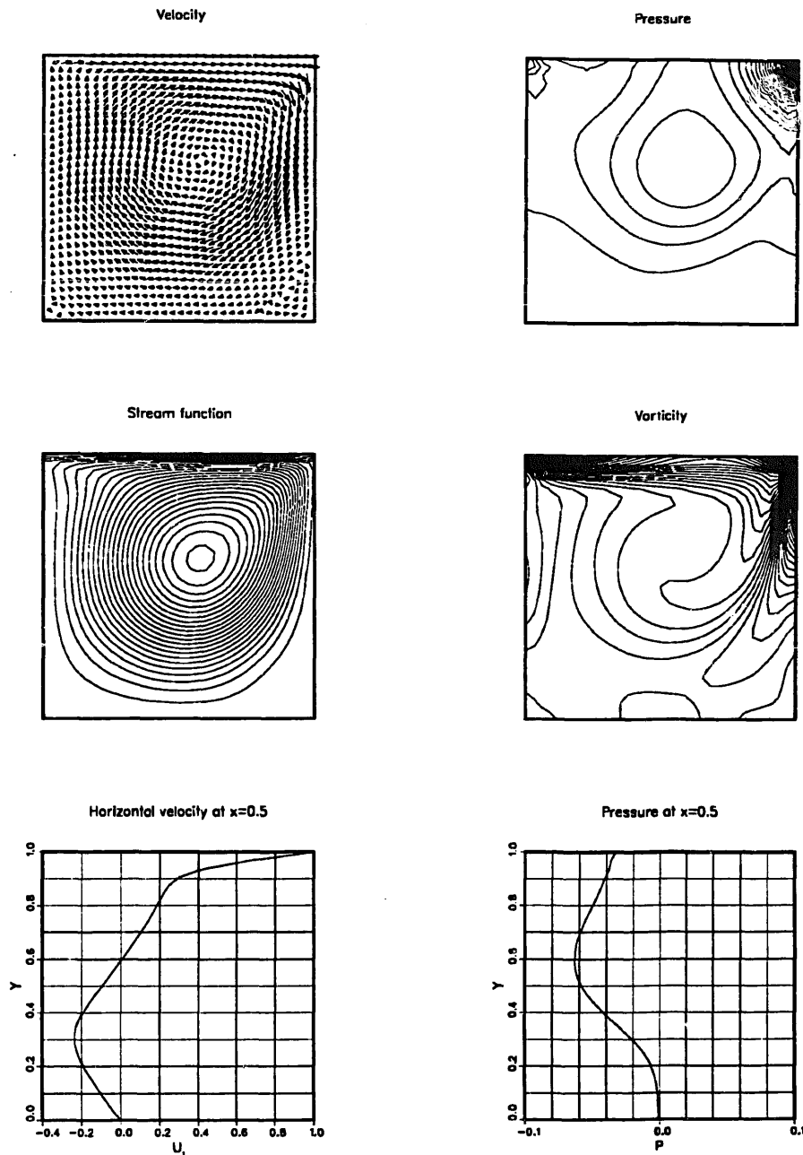
Fig. 9. Driven cavity flow at Reynolds number 400: steady-state solution obtained with P1P1/T1.
