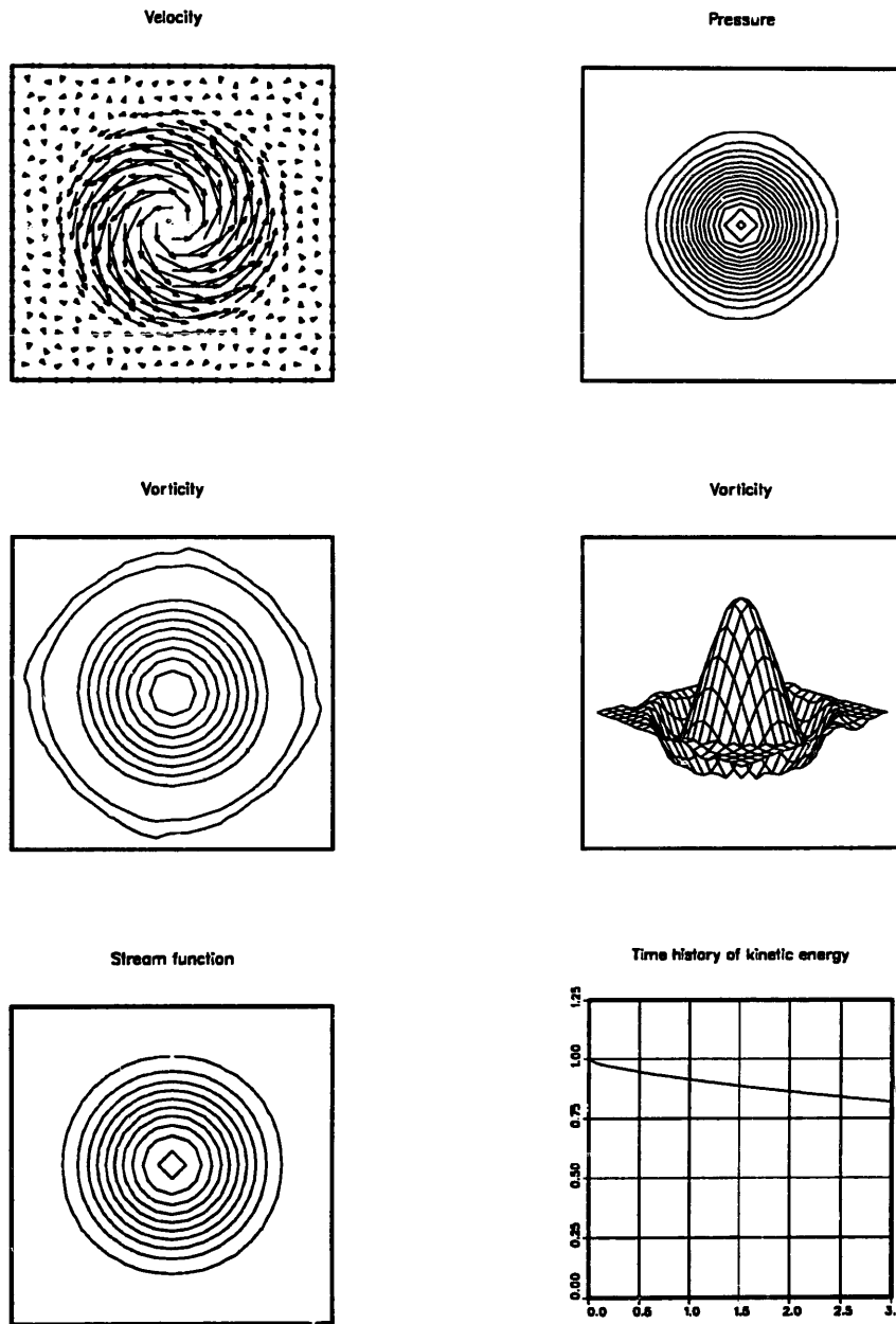
Fig. 7. Solution of the standing vortex problem at t = 3 with P1P1/T1 (with \tau as defined by (20)).
