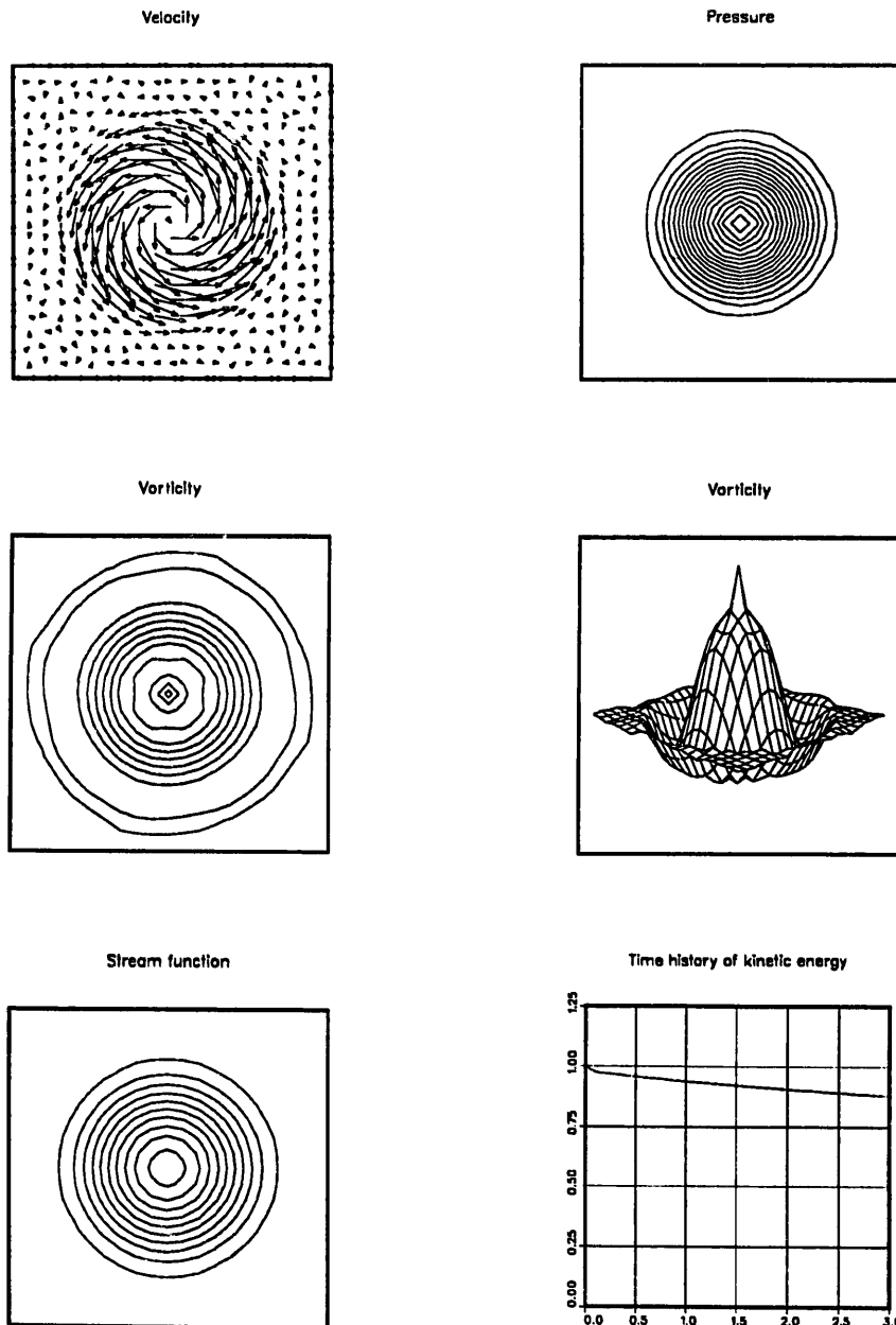
Fig. 2. Solution of the standing vortex problem at t = 3 with Q1Q1/T1.
