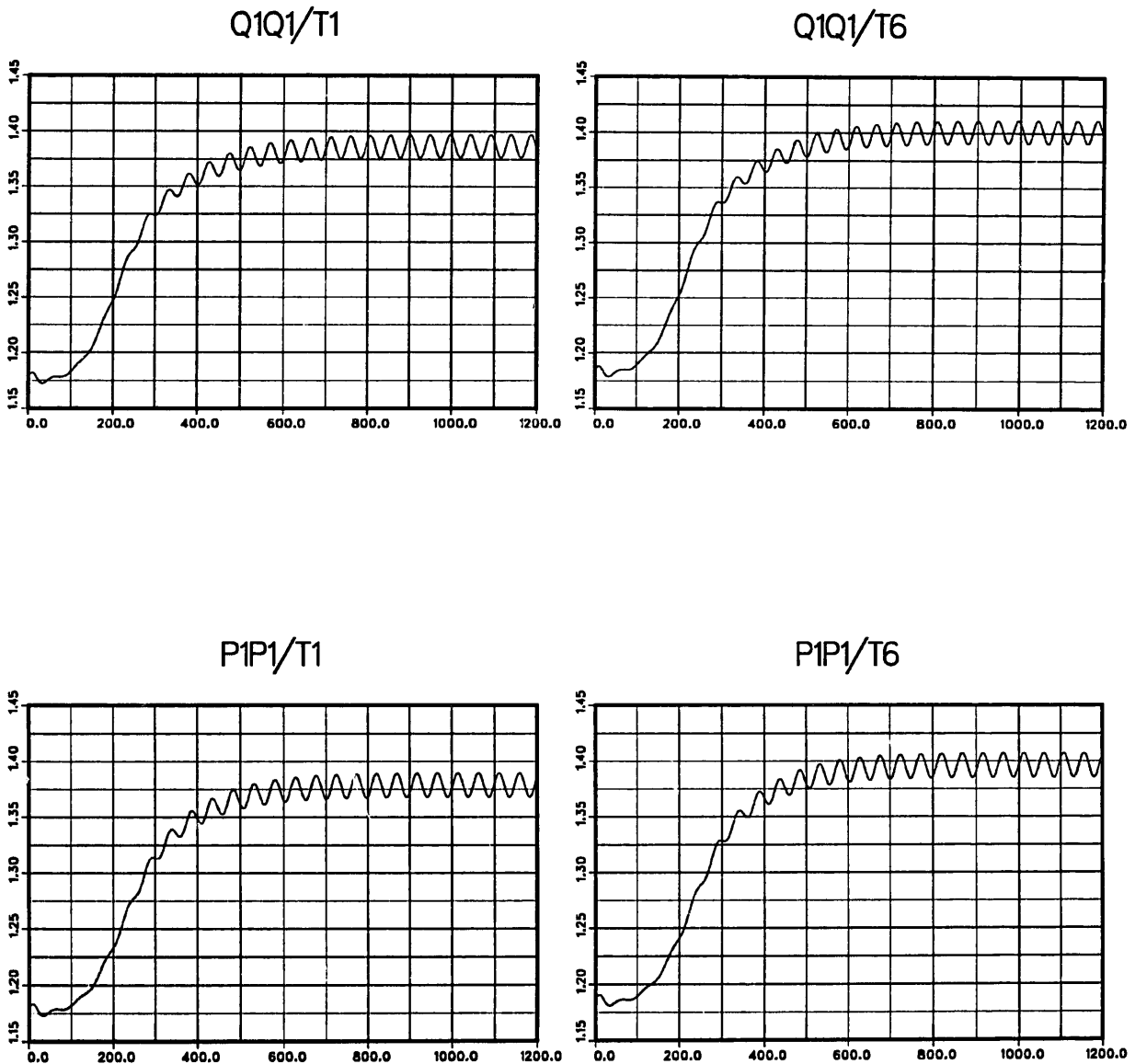
Fig. 11. Time history of the drag coefficient obtained with various elements.
