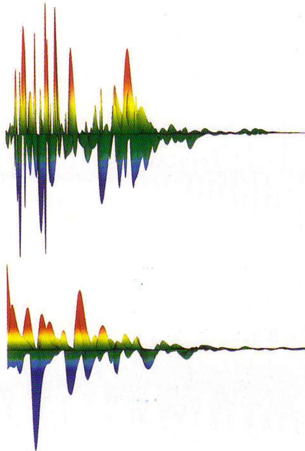
Fig. 8. 3D computation at Re=140 . Side view of the elevation plot for the streamwise component of the vorticity at the centered horizontal plane for SD-2 (upper) and SD-3 (with different scale) (lower). The color indicates the value of the vorticity (red: positive, blue: negative).
