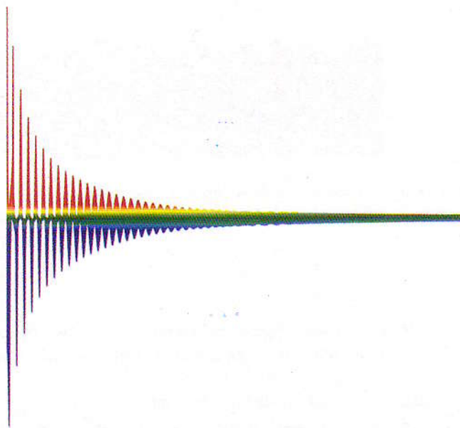
Fig. 4. 2D computation at Re=140 . Side view of the elevation plot for the vorticity for SD-2. The color indicates the value of the vorticity (red: positive, blue: negative).
