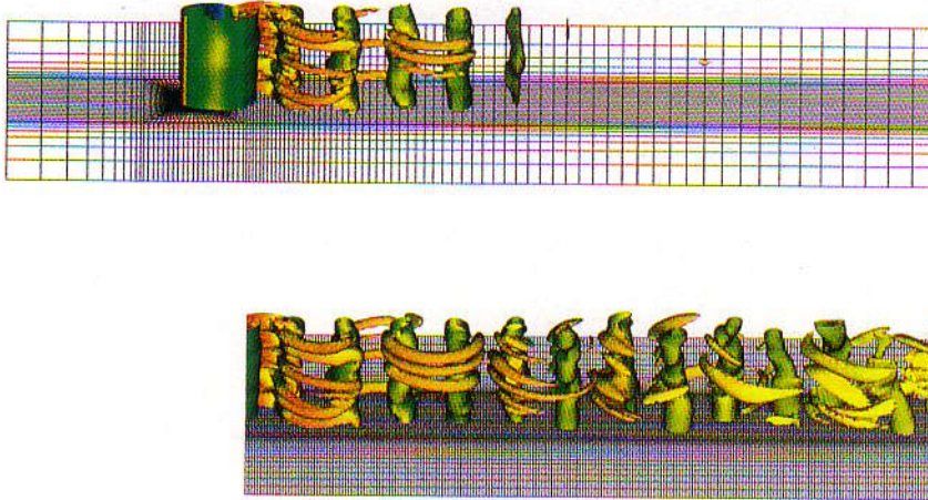
Fig. 1. Re=300 : effect of mesh refinement. The isosurfaces corresponding to the 0.5 value of the vorticity magnitude. Obtained with the single-domain (upper) and multi-domain (lower) computations.
